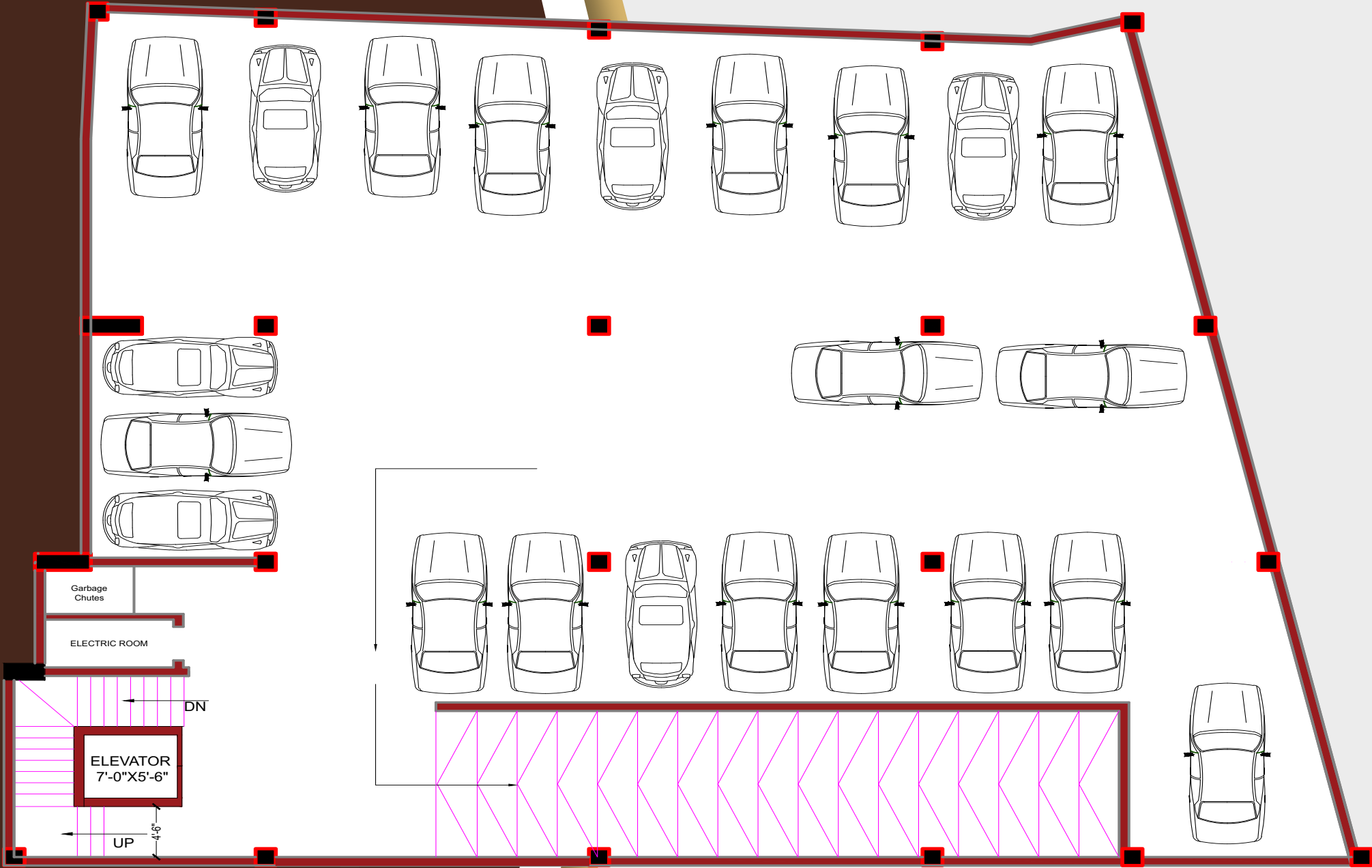
BASEMENT 2 FLOOR PLAN
