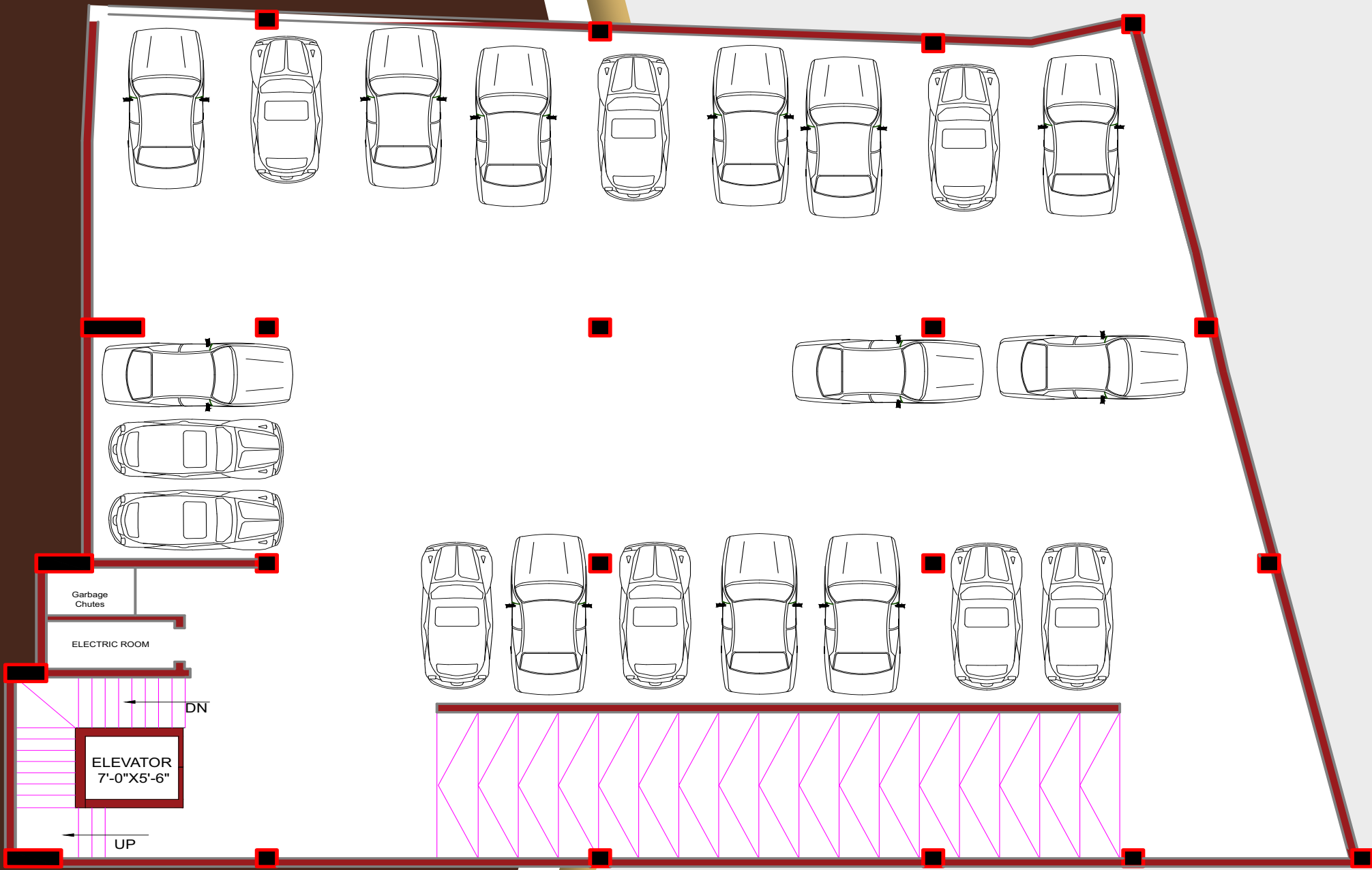
BASEMENT 1 FLOOR PLAN
